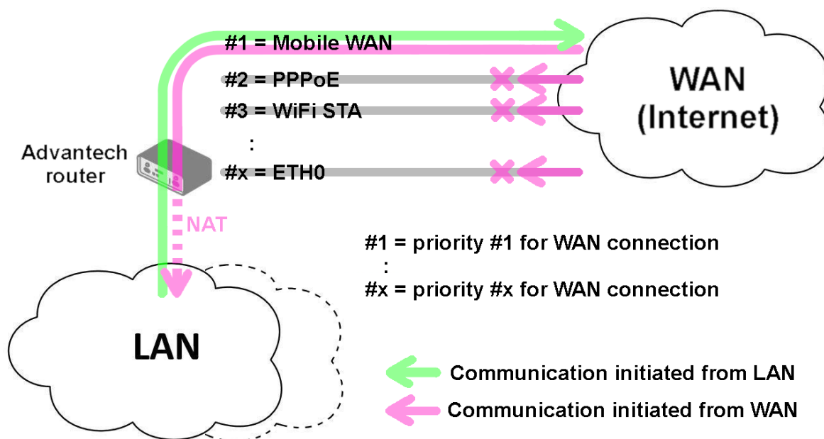
Figure 33: Example #1: Topology
